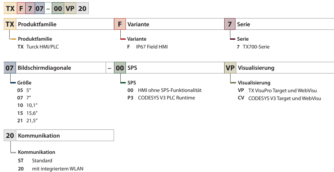
Abb. 2: Typenschlüssel TX700
