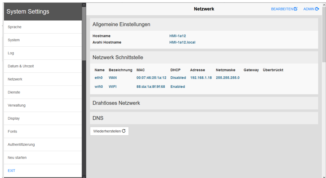
Abb. 7: Webserver – System Settings
