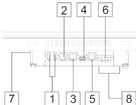
Abb. 10: TX7...FB – Anschlüsse
