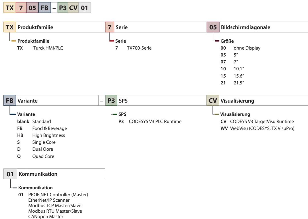
Abb. 2: Typenschlüssel TX700
